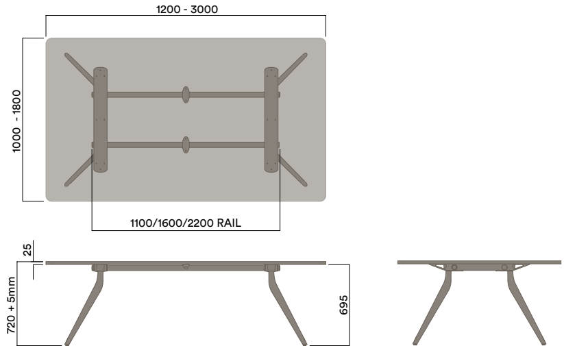
E-1211-XL, E-1216-XL, E-1222-XL 720 (standard Height)
