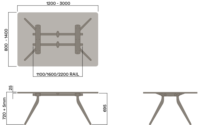
E-1211-XL, E-1216-XL, E-1222-XL 720 (standard Height)
