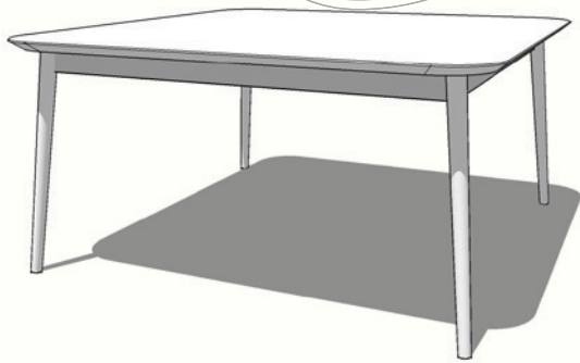
OEUF TABLE 1500sq x 740h SHAPED CHAMFER TOP + TAPER LEG
