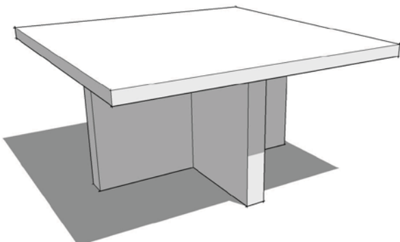
MD TABLE 1500sq x 740h 60TOP + PEDESTAL BASE
