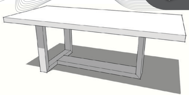
MD TABLE 2100 x 950 x 740h 60TOP + TBASE
