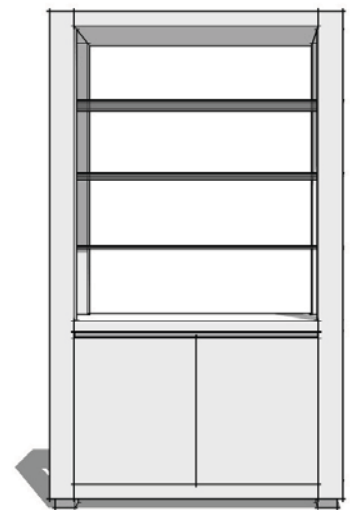
BOOKCASE 1200 x 400 x 2050h 3GLASS SHELF + 2DOOR LIGHTS
